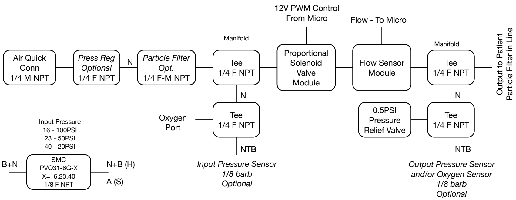
(S) SMC Valve Option
