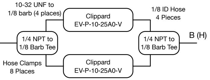
(SC) Small Clippard Valve Option
